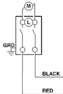
Wiring Diagram Double-Pole Pilot
